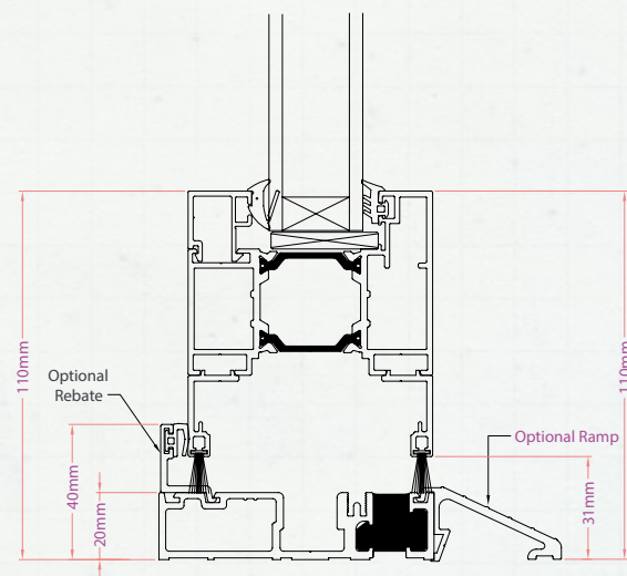
LOW THRESHOLD (WITH OPTIONAL RAMP & REBATE)
