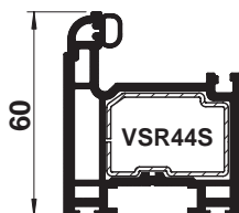
Standard Sash
